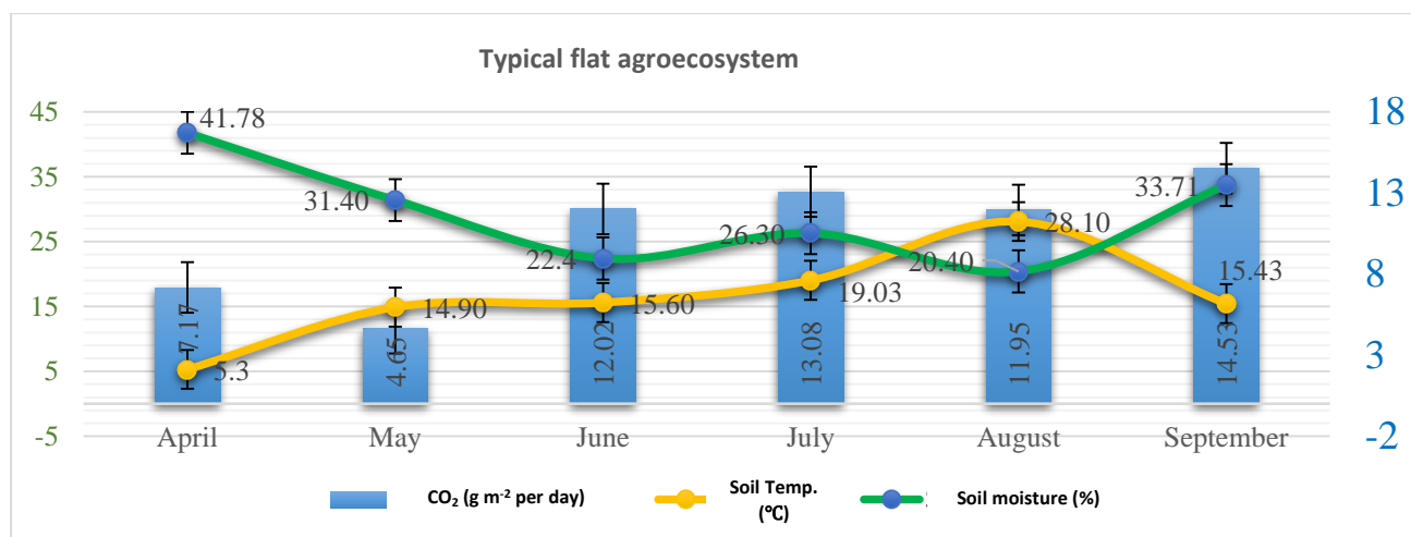
Fig. 4. Dynamics of the CO 2 emission of the typical flat agroecosystem
