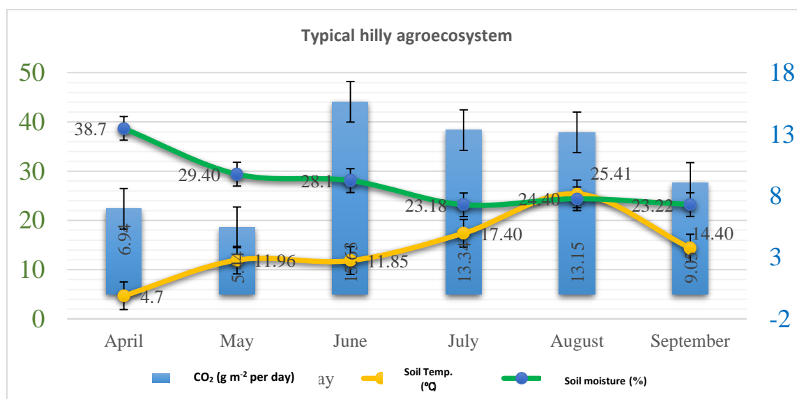
Fig. 3. Dynamics of the CO 2 emission of the typical hilly agroecosystem.
