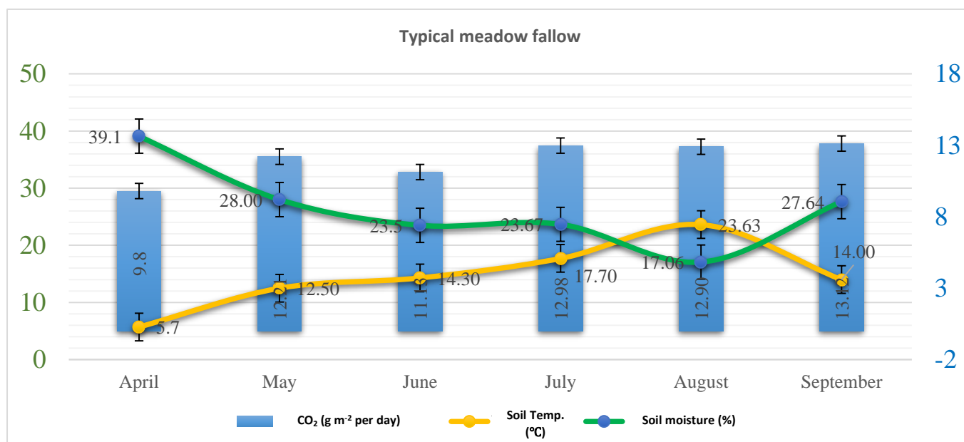
Fig. 5. Dynamics of CO 2 emissions from meadow fallow ecosystems.
