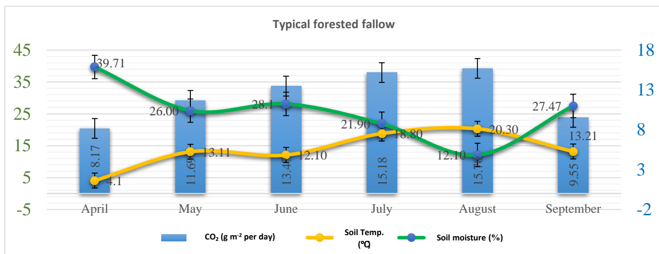
Fig. 6. Dynamics of CO_2 emission of forested fallow soils.
