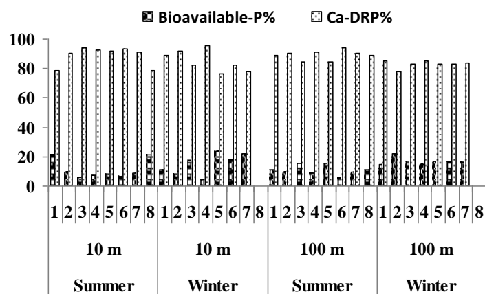
Fig. 2. Percentage of Bioavailable-P and Ca-DRP at different depths and seasons in the southern Caspian Sea surface sediment (2010-2011).
