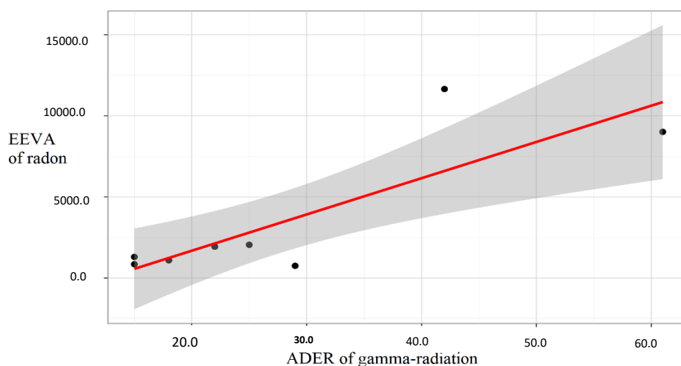
Fig. 3. Graph of the regression function characterizing the dependence of the indicator "EEVA of radon" on the indicator "ADER of gamma radiation".
