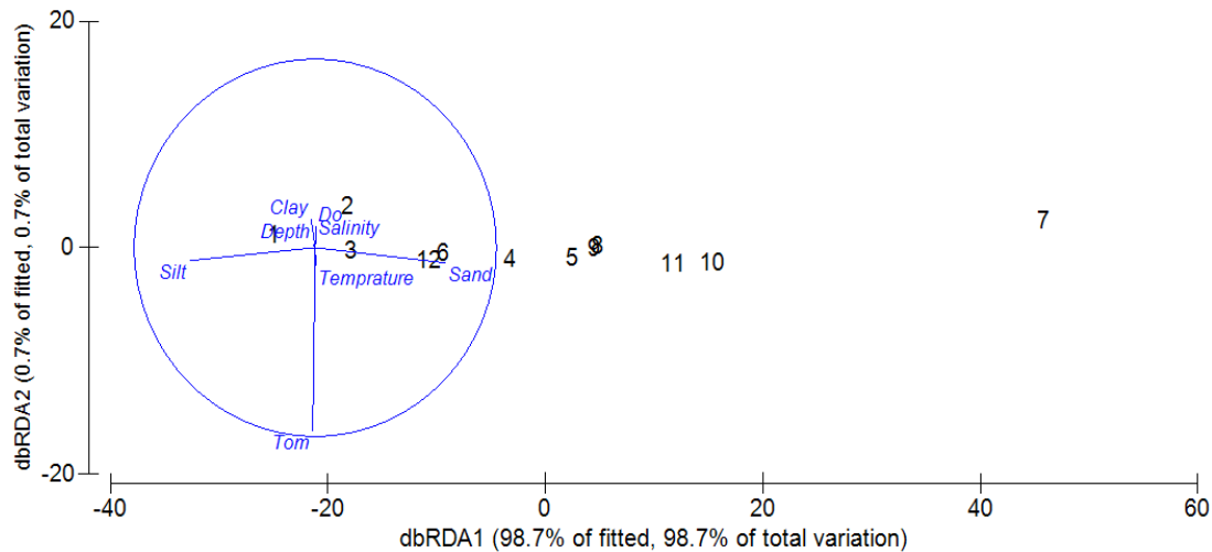
Fig. 8. A distance-based redundancy analysis (dbRDA) ordination of study samples by the macrobenthic assemblage structure.
