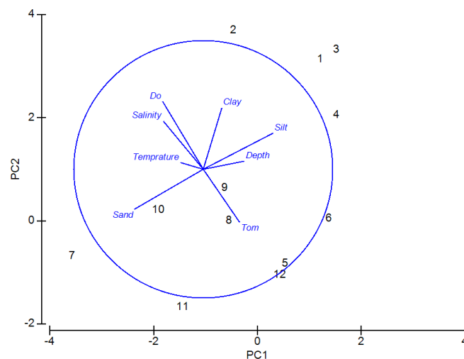
Fig. 3. Principal component analysis (PCA): spatial presentation of the study stations based on environmental data.
