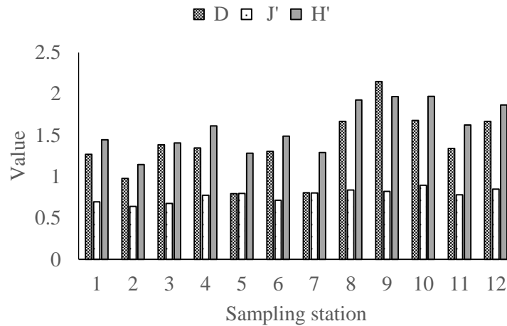
Fig. 6. Margalef richness index (D), Pielou's evenness index (J) and Shannon-Wiener diversity index (H 0 ) of each sampling station.
