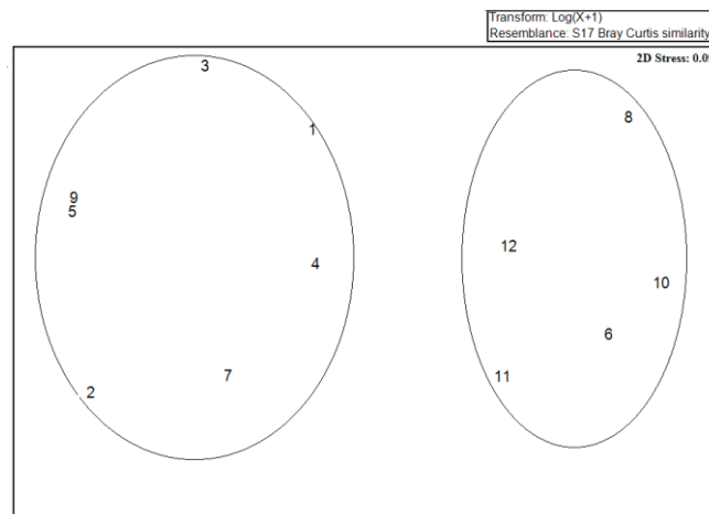
Fig. 7. Non-metric multidimensional (nMDS) plot of macrobenthic communities (based on Bray-Curtis similarity and log (X+1) transformed data on macrobenthic species).
